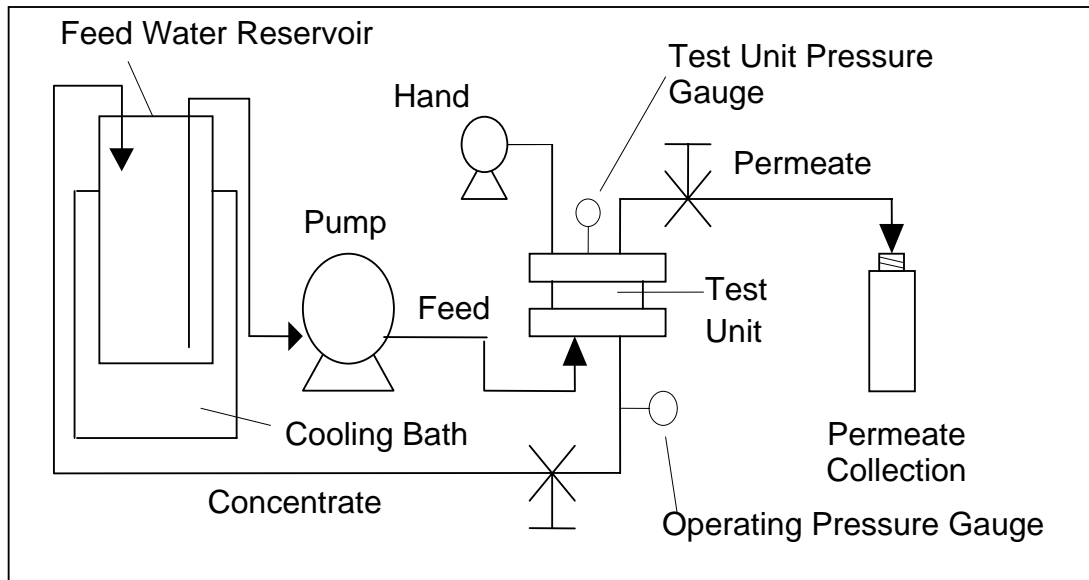
Figure 1: Filtration Assembly
